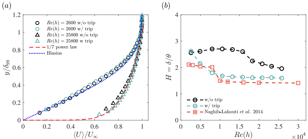
FIGURE 2. (a) Mean boundary layer profiles for sample cases of laminar and turbulent flow with and without tripwires at x = -3h and (b) the associated shape factors H = \delta/\theta showing when the transition to turbulence occurs.
