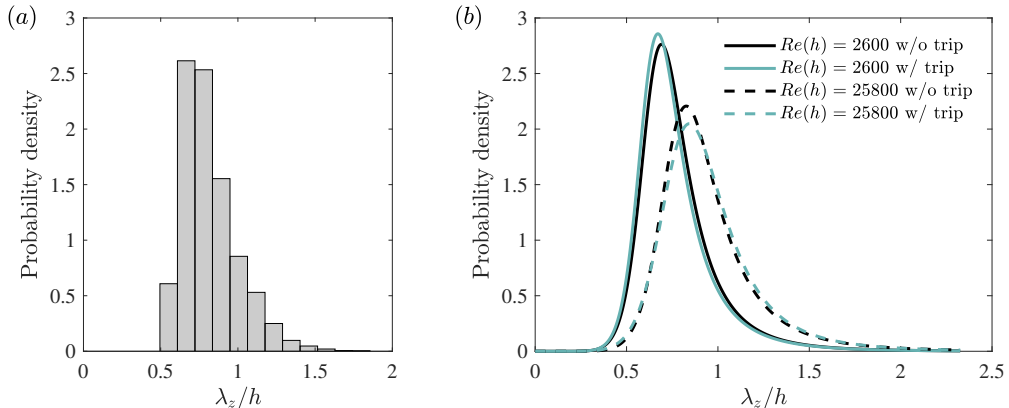
FIGURE 5. (a) Sample histogram of the wavelength of the streamwise vortices ( \lambda_z ) at Re(h) = 2600 without tripwires and (b) the fit probability density functions of \lambda_z at the lowest and highest Re with and without tripwires.
