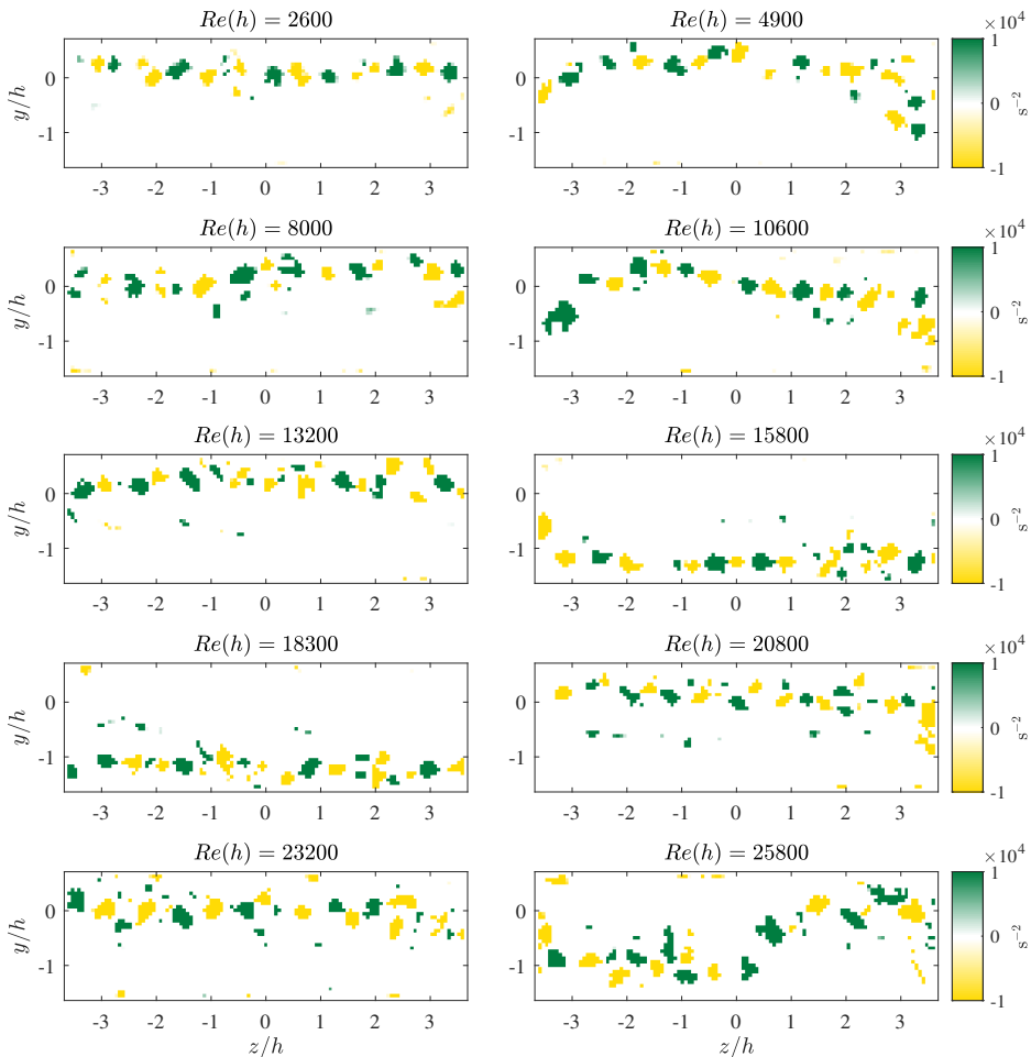
FIGURE 4. Snapshots of the modified Q -criterion ( Q' = \omega_x Q / |\omega_x| ) in the wake at x = 2h for all Re ; from the uncorrelated and untripped data set.
