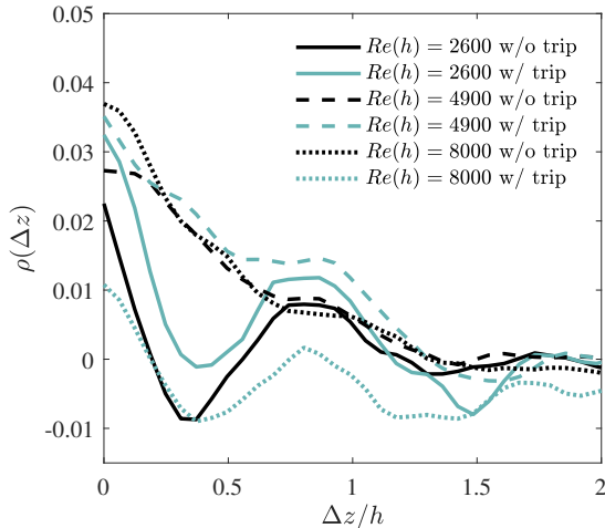
FIGURE 9. Cross-correlation coefficient calculated using equation 3.2 for Re(h) = 2600 , 4900, and 8000, with and without tripwires.
