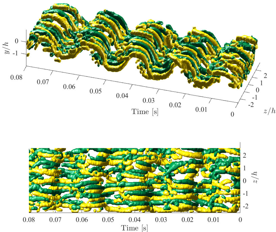
FIGURE 8. Isosurface construction of modified Q -criterion ( Q' = \omega_x Q / |\omega_x| ) in the wake at x = 2h for Re(h) = 2600 without tripwires. Green and gold represent positive and negative rotational directions, respectively. The isosurface was set to Q' = \pm 1500 \text{ s}^{-2} . A second-order regression filter with a kernel size of 3 has been applied to the data to reduce noise.
