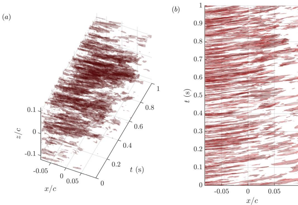
FIGURE 13. (a) Isosurfaces of the fluctuating streamwise velocity corresponding to u/U_\infty = 0.12 . (b) The isosurfaces projected onto the x-t axis to highlight the advection velocity of streaks in the streamwise direction.
