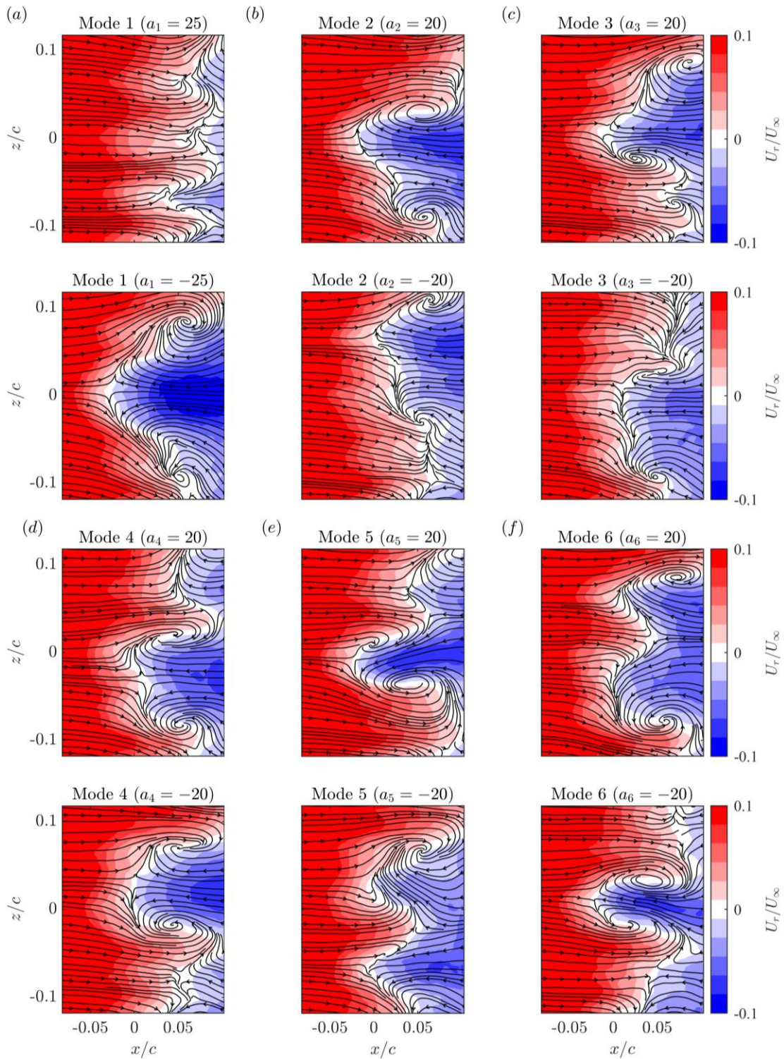
FIGURE 16. Low-order flow fields obtained by superimposing a selected spatial mode with the mean velocity field. The temporal amplitudes a_i are chosen based on the RMS value of the amplitudes associated with the respective mode. The background contours correspond to the normalized streamwise velocity.
