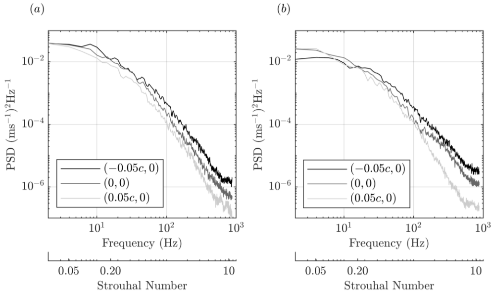
FIGURE 7. Power spectral density (PSD) of the fluctuating (a) streamwise and (b) spanwise velocity at a location upstream of the mean separation point ( x/c = -0.05 ), at the saddle point ( x/c = 0 ), and a point in the backflow region ( x/c = 0.05 ) along mid-span ( z = 0 ).
