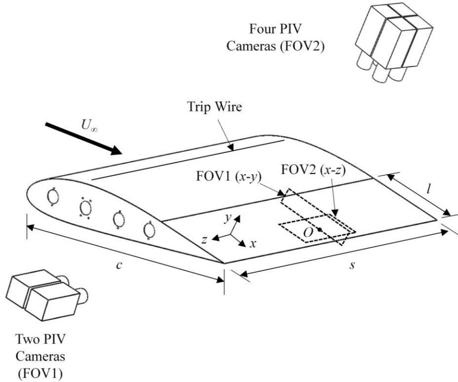
FIGURE 1. Schematic of the experimental setup and PIV fields-of-view. The coordinates are defined relative to the flat surface of the airfoil. The origin of the coordinate system ( O ) is located at the separation point at mid-span and 140 mm ( 0.14c ) upstream of the trailing edge. Note that the axes are displaced from mid-span of the airfoil for clarity of the figure.
