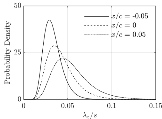
FIGURE 12. Probability density functions (PDFs) of the spanwise wavelength of high-speed streaks ( \lambda_z/s ) at three different chordwise positions. The wavelengths were determined by spatial autocorrelation of the fluctuating streamwise velocity using Eq. (4.1) and were fitted with a lognormal distribution.
