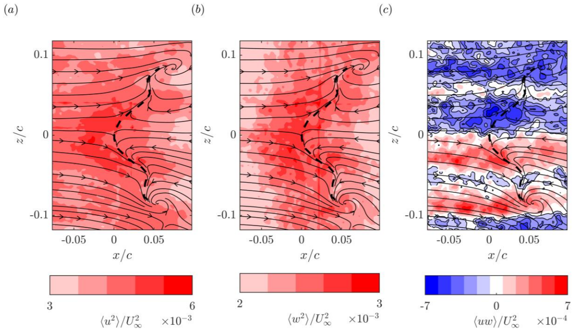
FIGURE 6. Contours of (a) streamwise and (b) spanwise components of Reynolds normal stress, and (c) Reynolds shear stress in the x - z plane. The near-surface streamlines obtained from the mean flow are superimposed on the contours. The negative contours are shown with solid black outlines.
