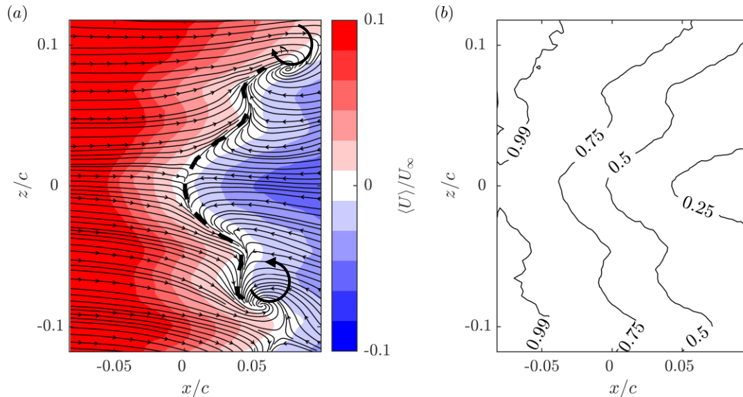
FIGURE 5. (a) Streamlines obtained from the mean flow in the near-surface ( y = 2 mm) plane. Colors in the background represent the mean streamwise velocity normalized by freestream speed of the wind tunnel U_\infty . The positive and negative contours can be identified based on the streamwise direction of the streamlines. (b) Contour lines of the backflow parameter ( \gamma ) in the near-surface plane, showing intermittency of the separated flow.
