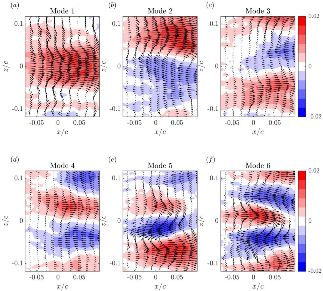
FIGURE 15. The first six POD modes obtained from decomposition of the fluctuating velocity field. Contours of the fluctuating streamwise velocity are shown in the background.
