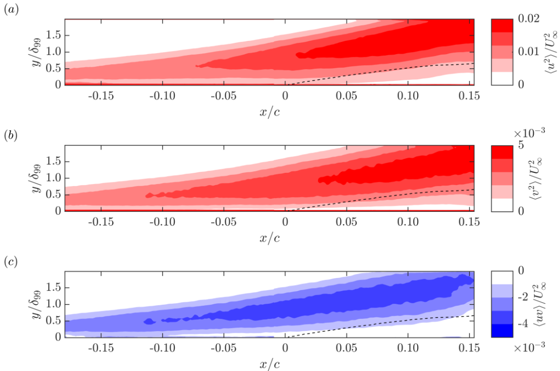
FIGURE 3. Contours of (a) streamwise (b) and wall-normal Reynolds stresses, and (c) Reynolds shear stress in the x - y plane. The dashed line shown in the figures indicates \langle U \rangle = 0 . The values are normalized using the freestream speed of the wind tunnel U_\infty .
