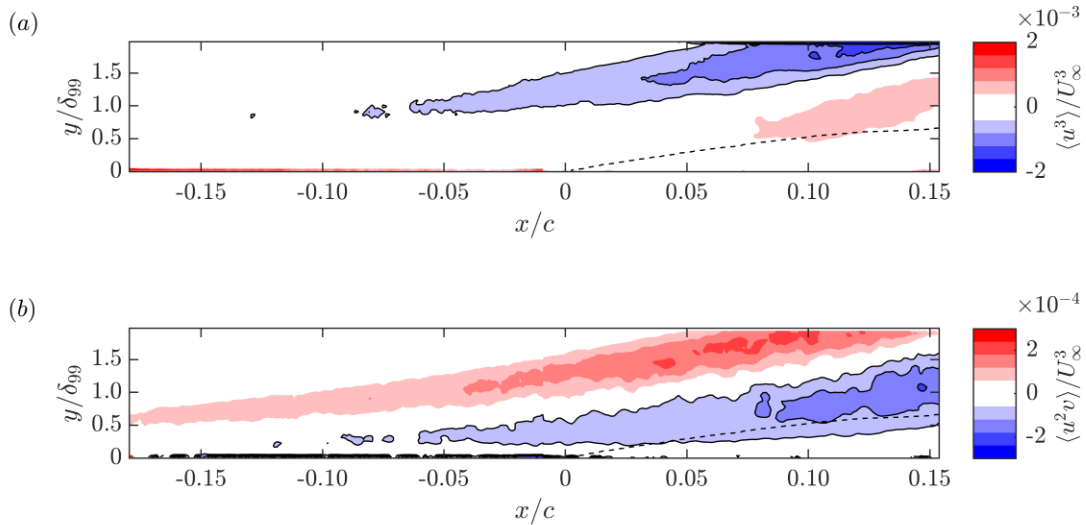
FIGURE 4. Contours of the third-order central moments (a) \langle u^3 \rangle / U_\infty^3 and (b) \langle u^2 v \rangle / U_\infty^3 in the x - y plane. The turbulence transport terms are normalized by the freestream speed of the wind tunnel U_\infty . The dashed line shown in the figures indicates \langle U \rangle = 0 . Contours enclosed with solid lines denote negative values and contours without solid borders denote positive values.
