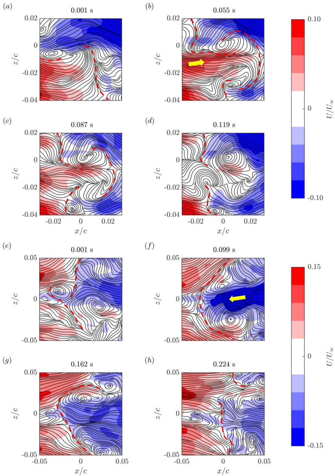
FIGURE 11. The formation and dissipation of (a – d) a forward stall cell and (e – h) a backward stall cell due to local concentrations of strong streamwise momentum. The colors in the background correspond to the normalized streamwise velocity. Videos of the process are provided in movies 2 and 3 of the supplementary materials online.
