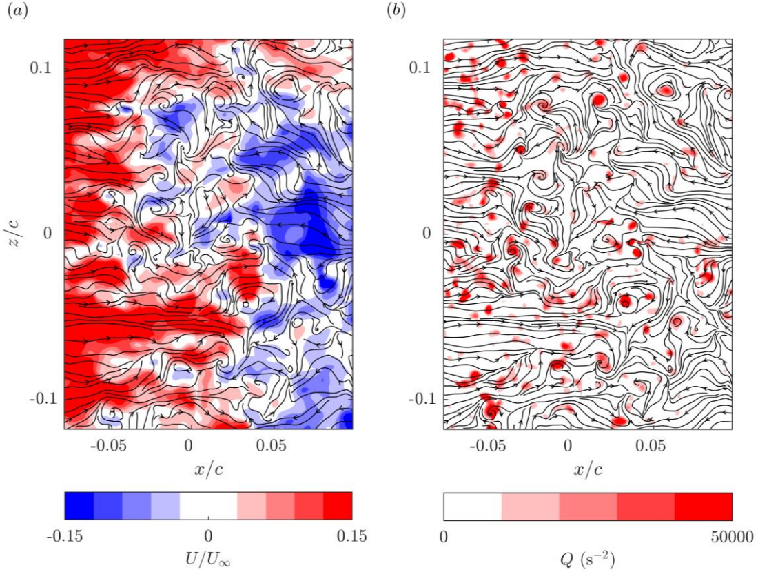
FIGURE 8. Snapshot of the instantaneous near-surface streamlines with a background contour of (a) normalized streamwise velocity and (b) two-dimensional Q -criterion. The sign of the contours in (a) can be identified using the streamwise direction of the streamlines.
