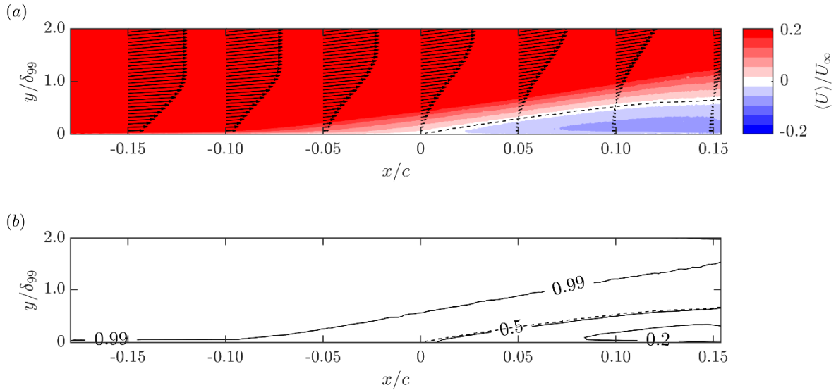
FIGURE 2. (a) Vectors of mean velocity at various chordwise positions upstream and downstream of the mean separation point ( x/c = 0 ). The vector profiles are shown in 0.05c increments and the vectors are downsampled by a factor of 6 in the y -direction for clarity of the visualization. Contours of the normalized mean streamwise velocity, \langle U \rangle / U_\infty , are shown in the background. Positive contours are above the dashed line and negative contours are located under the dashed line. (b) Contour lines of the backflow parameter ( \gamma ) in the x - y plane. The dashed line indicates where the mean streamwise velocity is zero.
