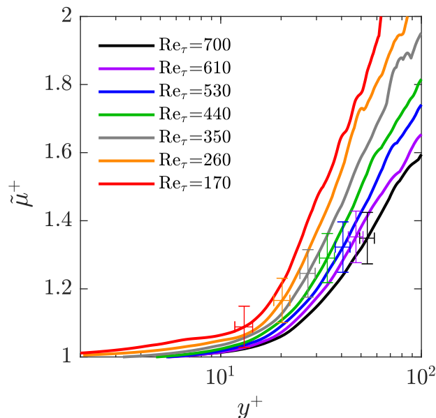
FIG. 7. The pseudo-mean viscosity normalized by wall viscosity as a function of inner-normalized wall location.
