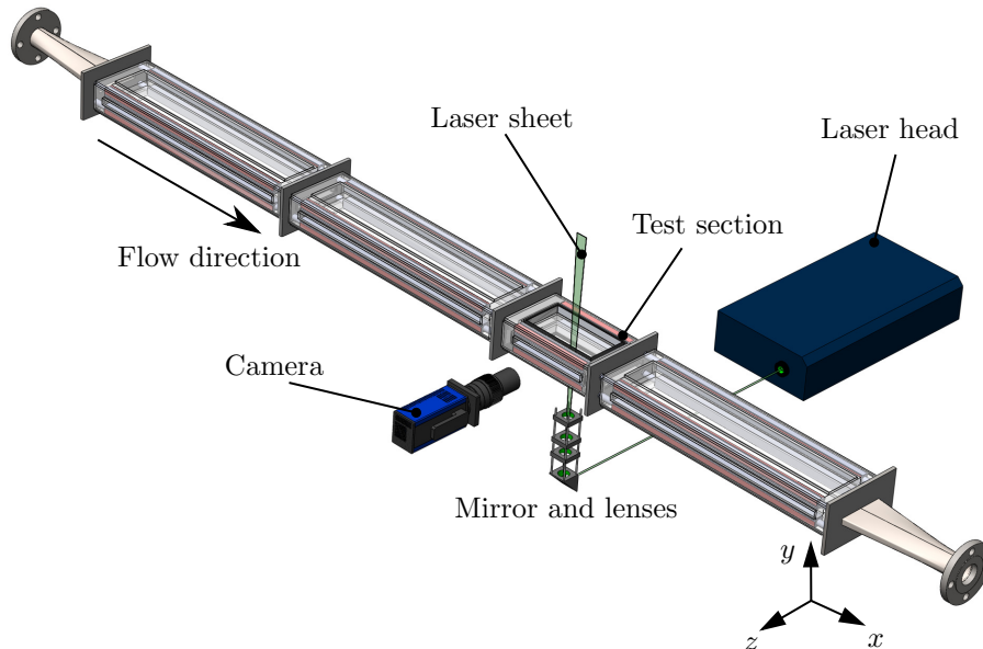
FIG. 3. Isometric 3D model of the planar PIV setup relative to the glass test section and channel section.
