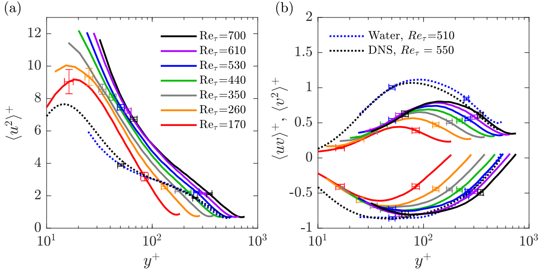
FIG. 13. Inner normalized profiles of (a) streamwise Reynolds stress, (b) wall-normal and Reynolds shear stresses, for flows with 170ppm XG solution.
