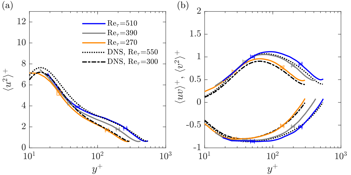
FIG. 5. Inner normalized profiles of (a) streamwise Reynolds stress, (b) wall-normal and Reynolds shear stresses, for Newtonian flows.
