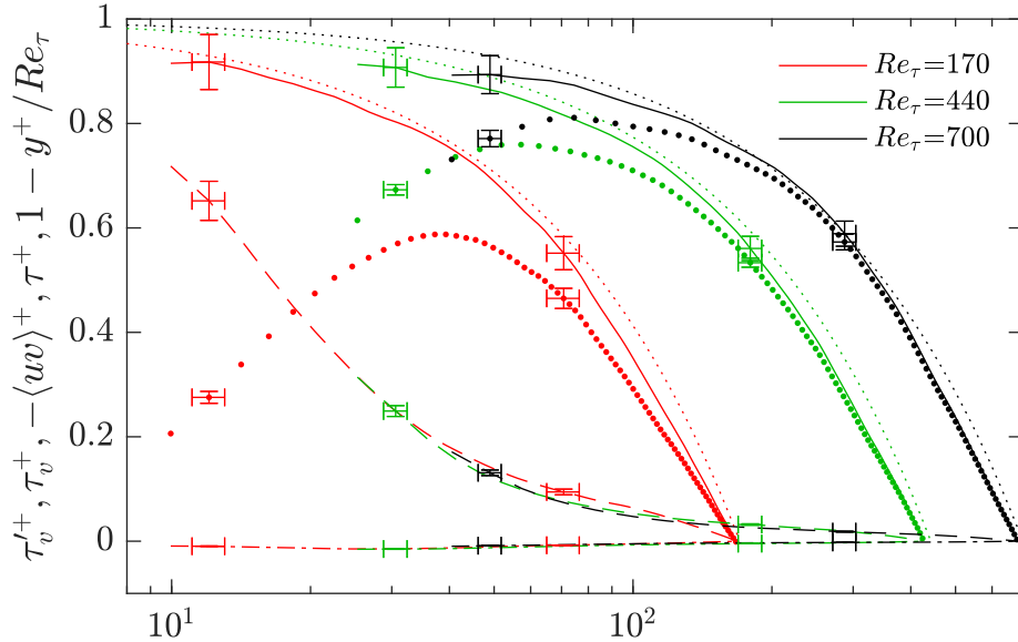
FIG. 14. Inner-normalized mean stress balance of XG at three of the seven Re_\tau conditions. The lines correspond to \dots 1 - y^+/Re_\tau , \text{— } \tau^+ , \cdot \langle uv \rangle^+ , \text{--- } \tau_v^+ , \cdot \tau_v'^+ . Error bars are shown at y/h of 0.07 and 0.42.
